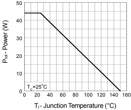
Power Dissipation
