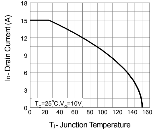
Drain Current
