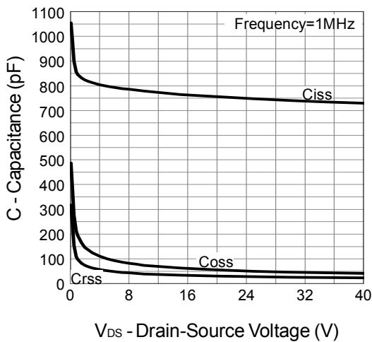
Capacitance
