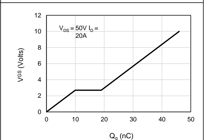
Figure 6: Gate-Charge Characteristics
