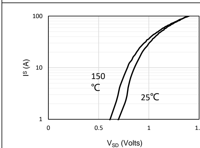
Figure 5: Body-Diode Characteristics
