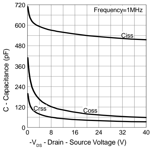
Capacitance
