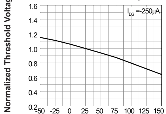
Gate Threshold Voltage
