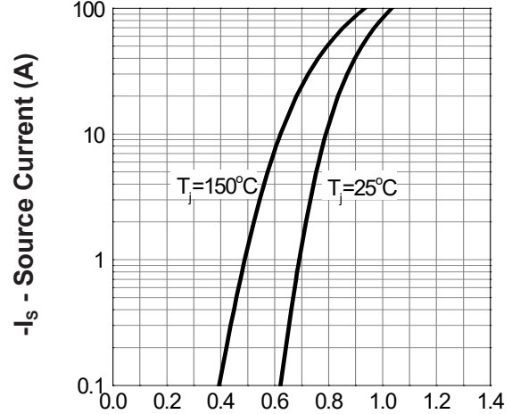
- V_{SD} - Source - Drain Voltage (V)
