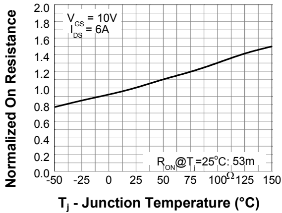
Normalized On Resistance
