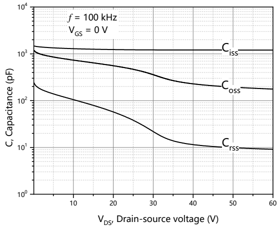
Figure 7. Typ. capacitances
