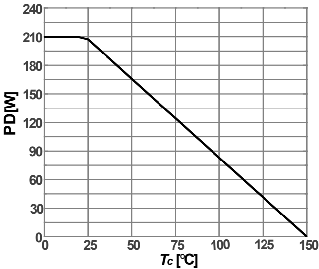
Diagram 1: Power dissipation
