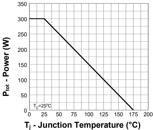
Power Capability
