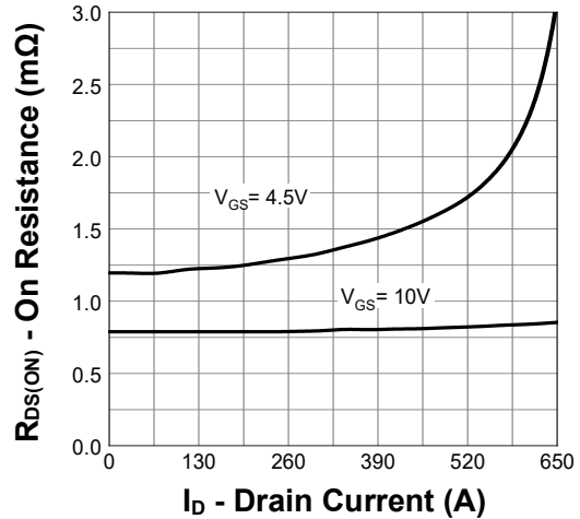
On Resistance
