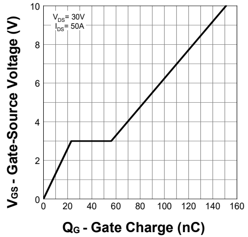
Gate Charge
