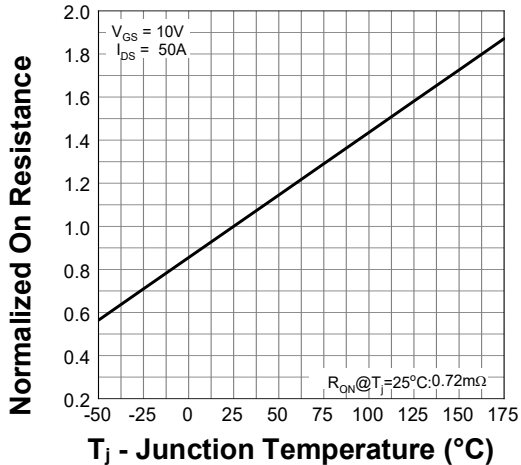
Normalized On Resistance
