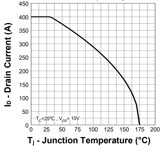
Current Capability
