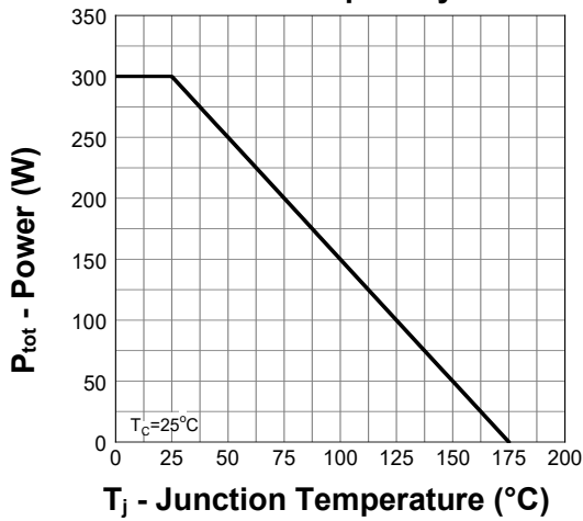
Power Capability
