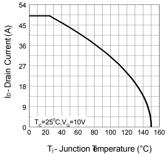
Drain Current
