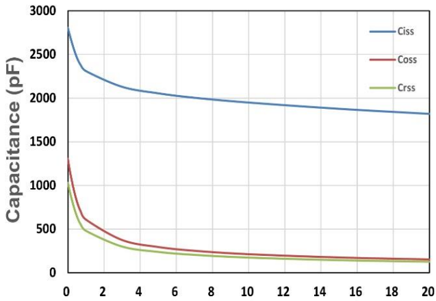
Figure 7. Capacitance
