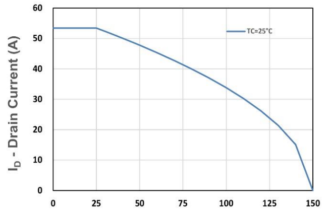
Figure 10. Drain Current
