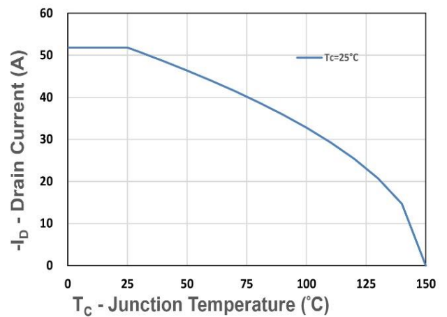
Figure 10. Drain Current
