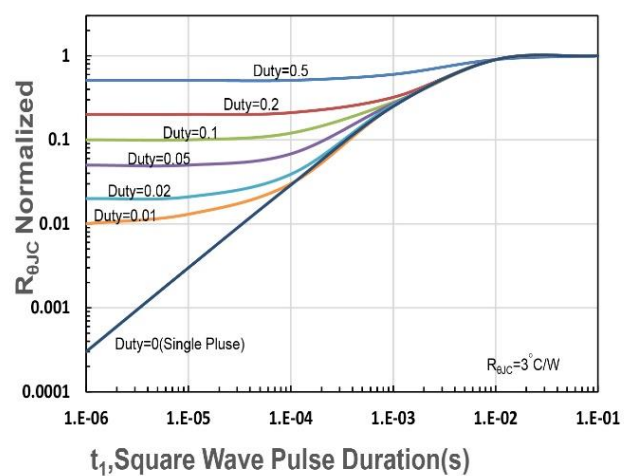
Figure 12. R θJC Transient Thermal Impedance
