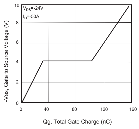
Figure 7. Gate Charge
