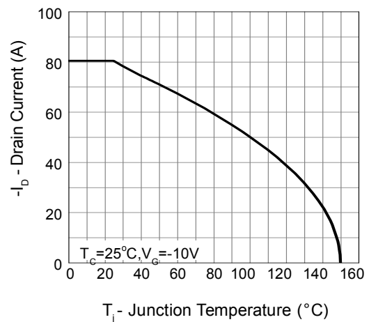
Drain Current
