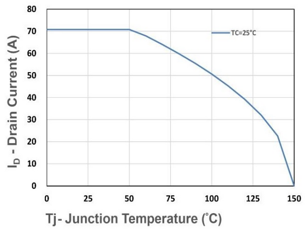
Figure 10. Drain Current
