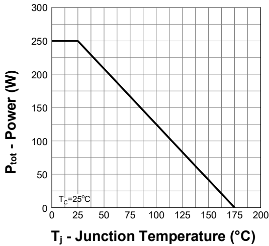
Power Capability
