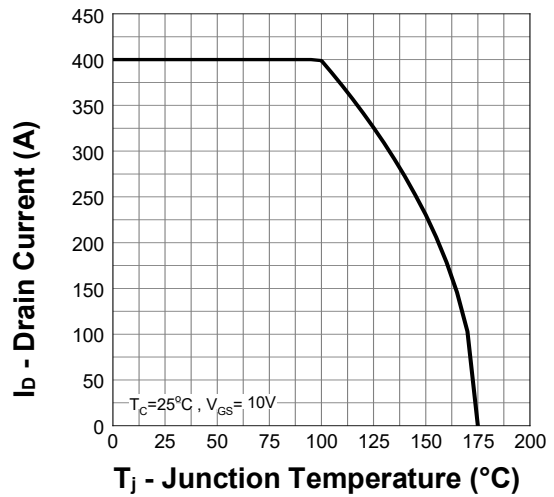
Current Capability
