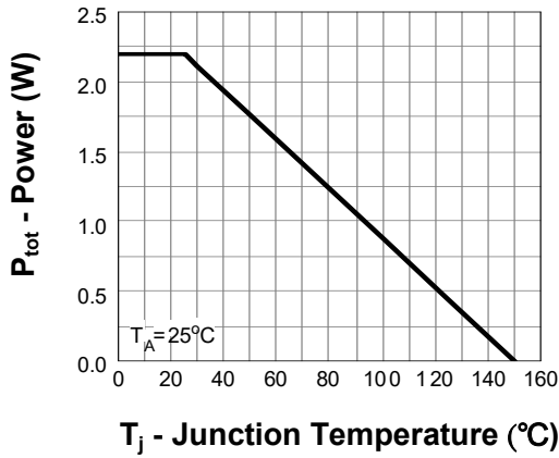
Power Dissipation
