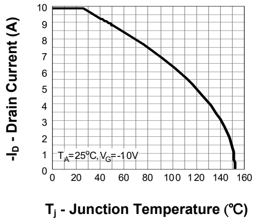
Drain Current
