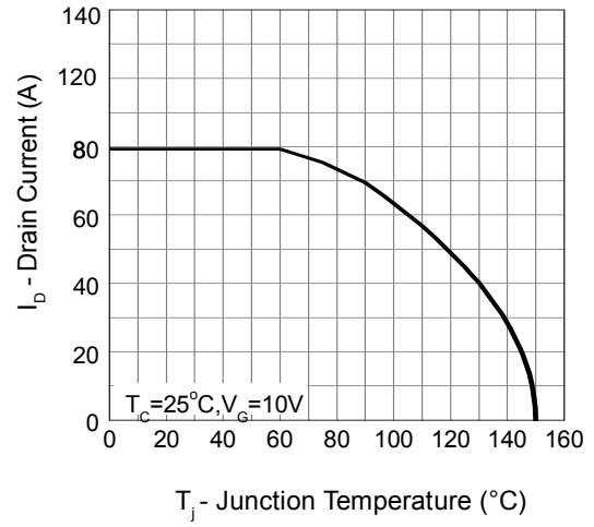
Drain Current
