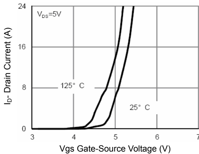
Figure 3 Transfer Characteristics
