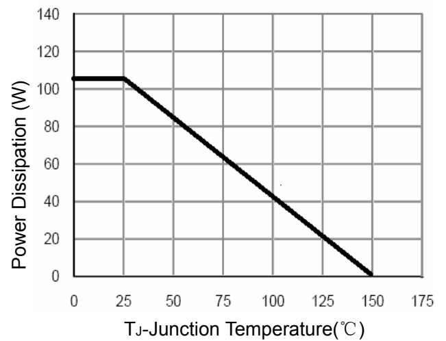
Figure 8 Power De-rating
