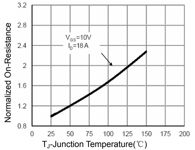
Figure 2 Rdson-Junction Temperature
