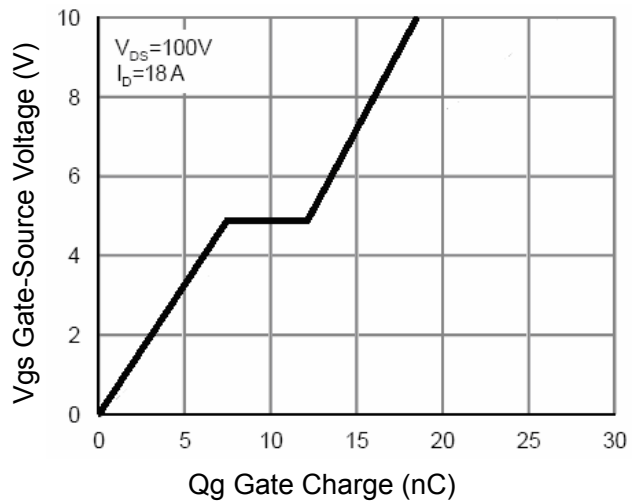
Figure 4 Gate Charge
