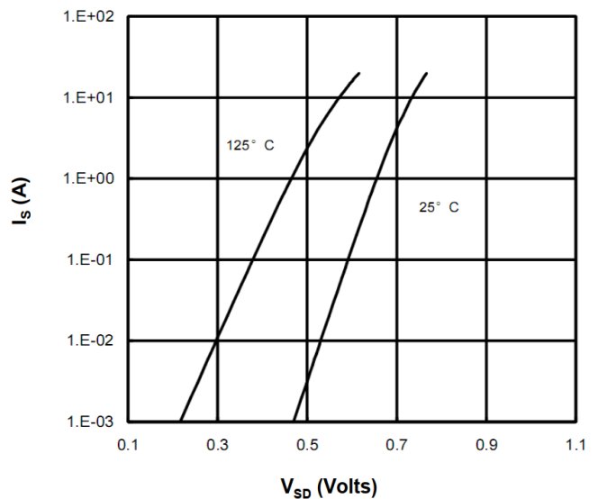
Figure 6: Body-Diode Characteristics
