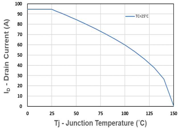
Figure 10. Drain Current
