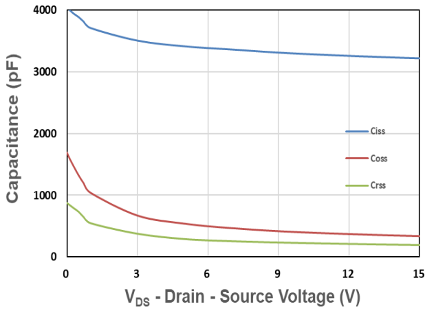
Figure 7. Capacitance
