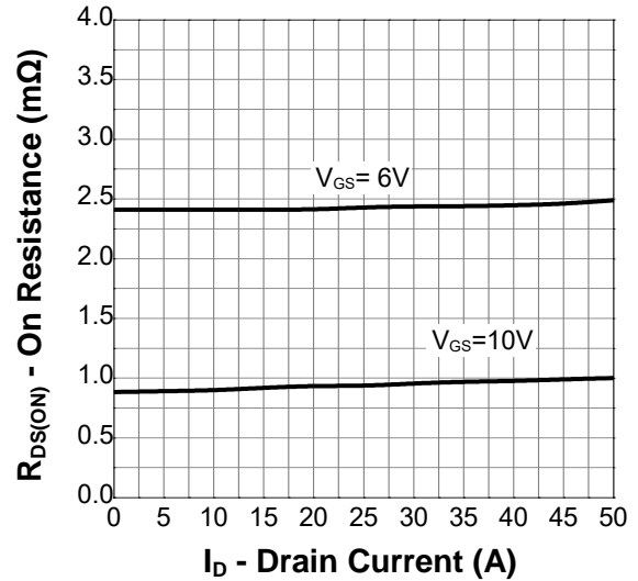
On Resistance
