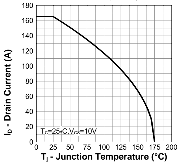
Current Capability
