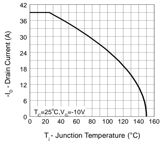
Drain Current
