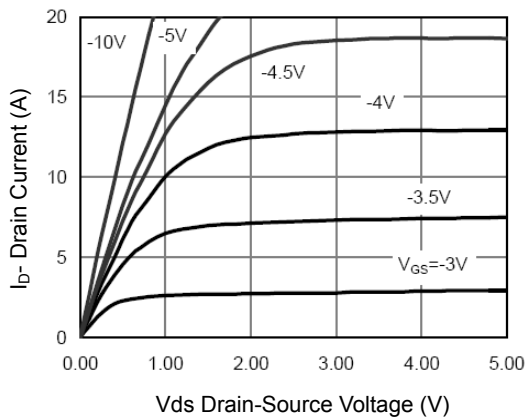
Figure 5 Output Characteristics
