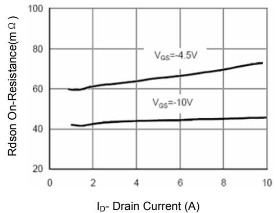
Figure 6 Drain-Source On-Resistance
