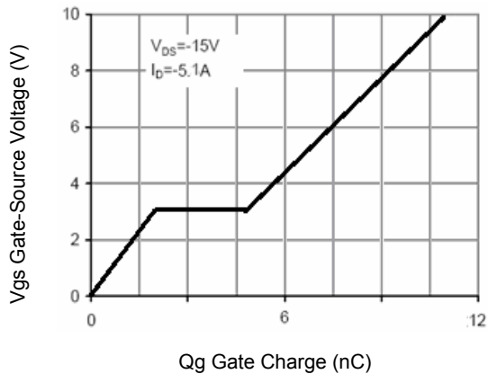
Figure 11 Gate Charge
