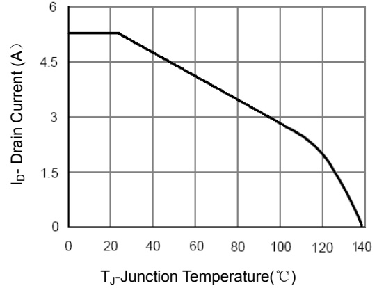
Figure 4 Drain Current
