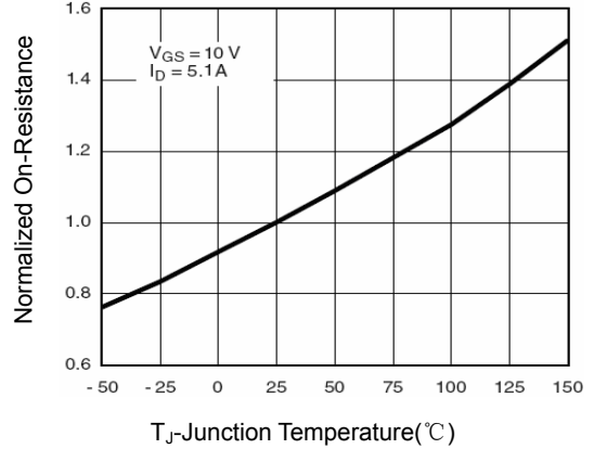
Figure 8 Drain-Source On-Resistance
