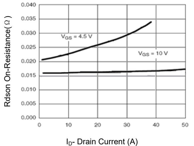
Figure 4 Drain-Source On-Resistance
