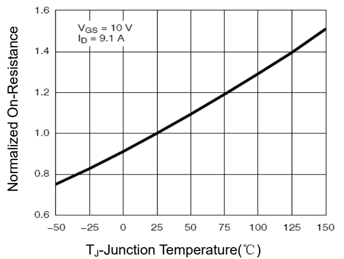
Figure 6 Drain-Source On-Resistance
