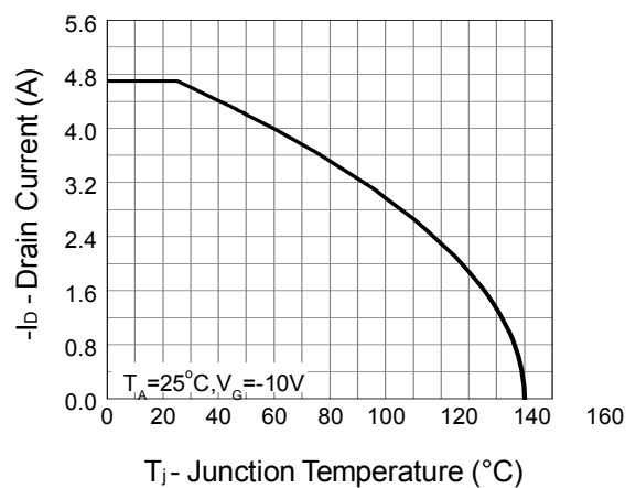
Drain Current
