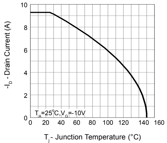
Drain Current
