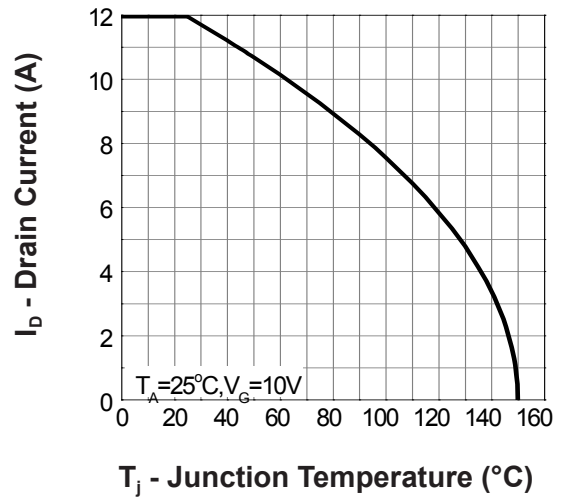
Drain Current
