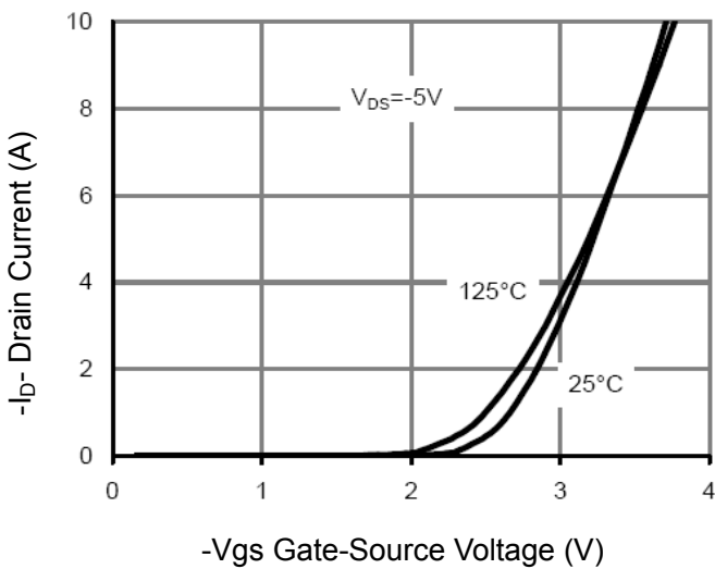
-V_{GS} Gate-Source Voltage (V) Figure 5 Transfer Characteristics
