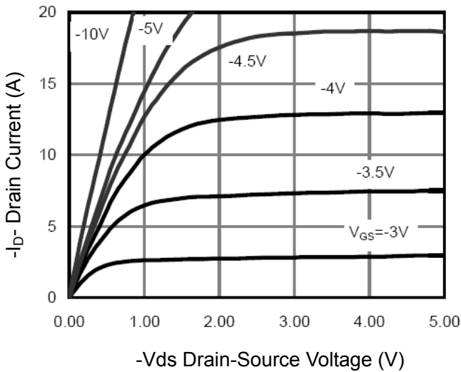
-V_{DS} Drain-Source Voltage (V) Figure 3 Output Characteristics
