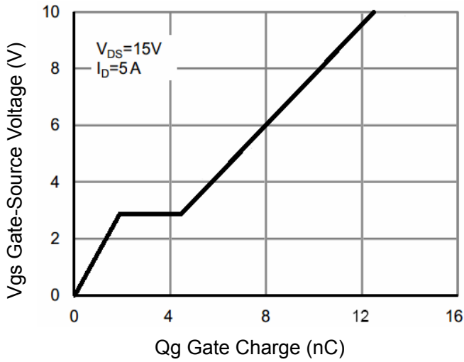
Figure 7 Gate Charge
