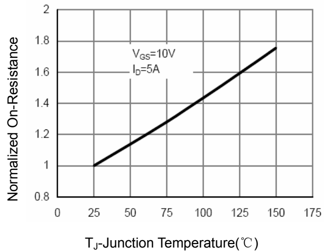
Figure 4 Drain-Source On-Resistance
