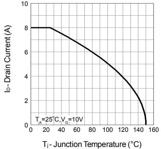
Drain Current
